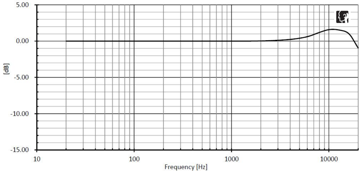
On-Axis Frequency Response(dB re 1V/Pa)
