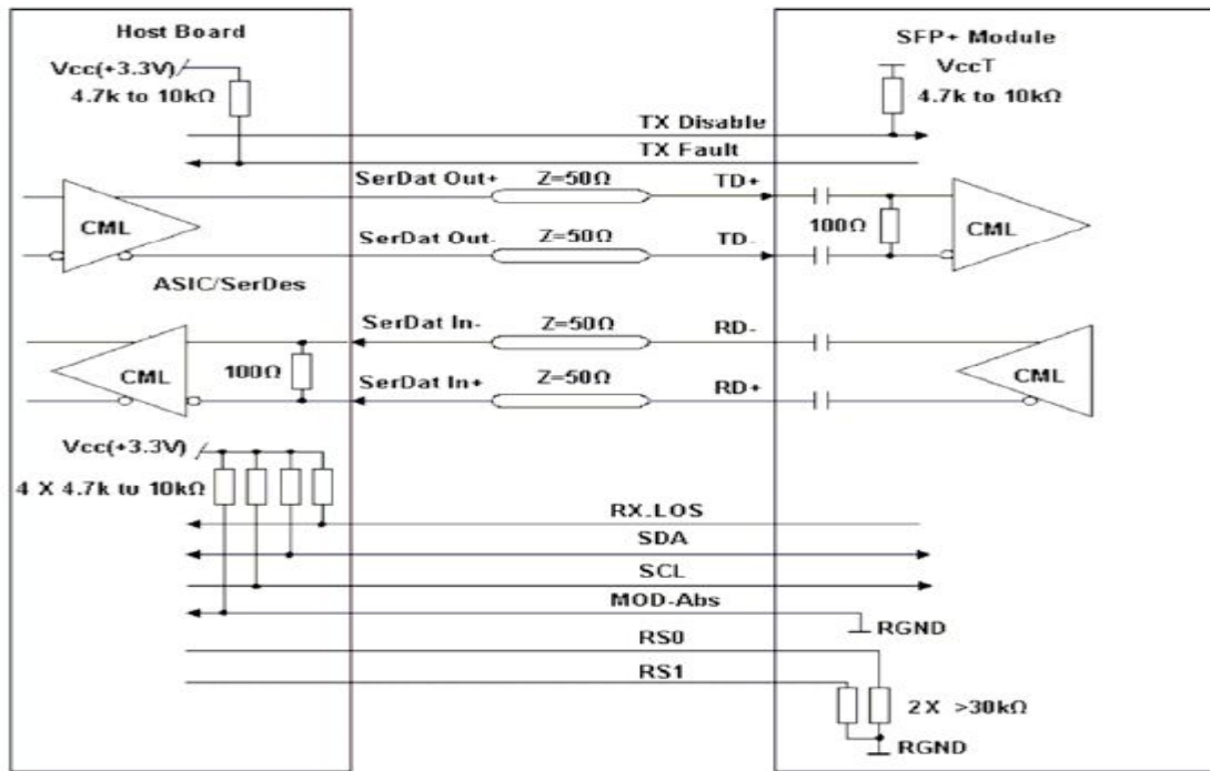
Figure 2, recommended interface circuit
