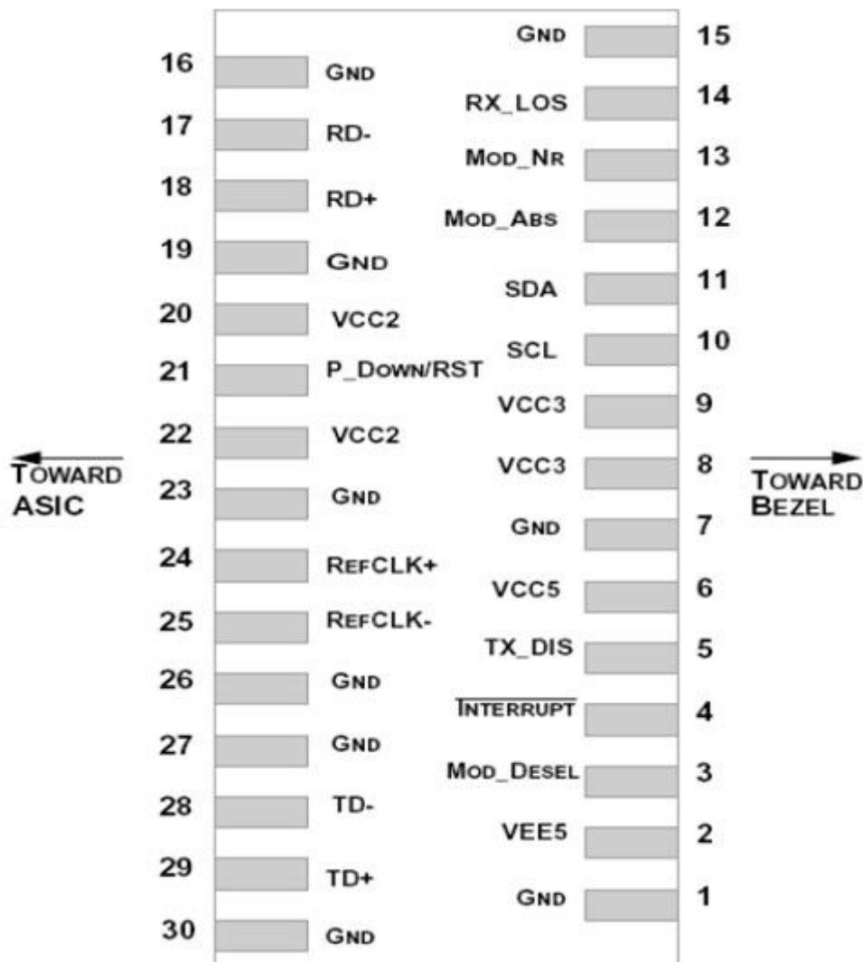
Figure 3,pins definitions
