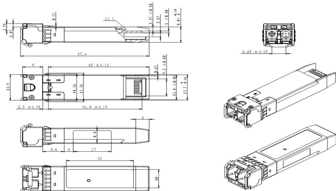
Figure 5, Mechanical Diagram
