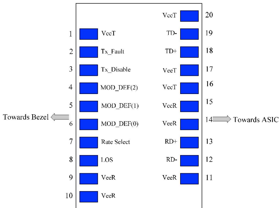
Figure 3, Pin View
