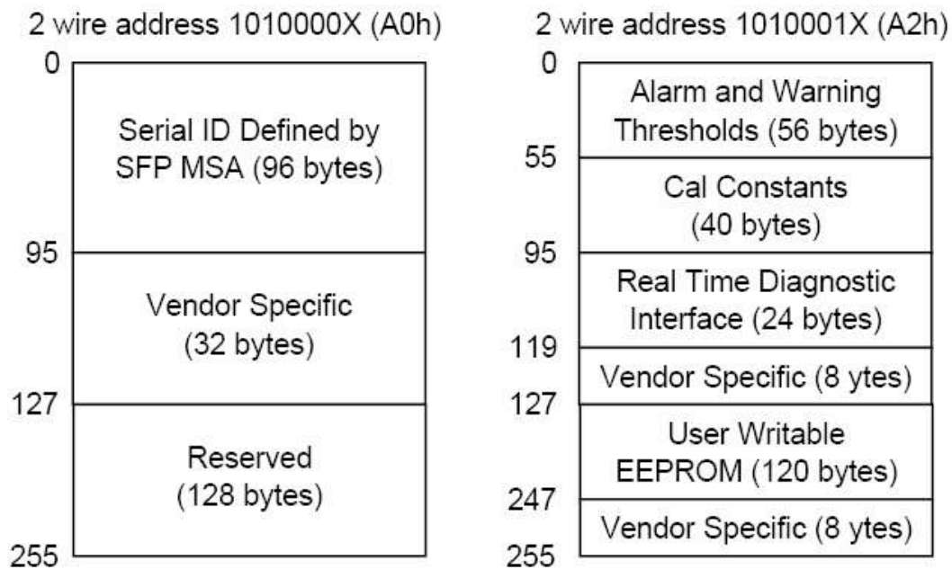
Figure 4, memory map
