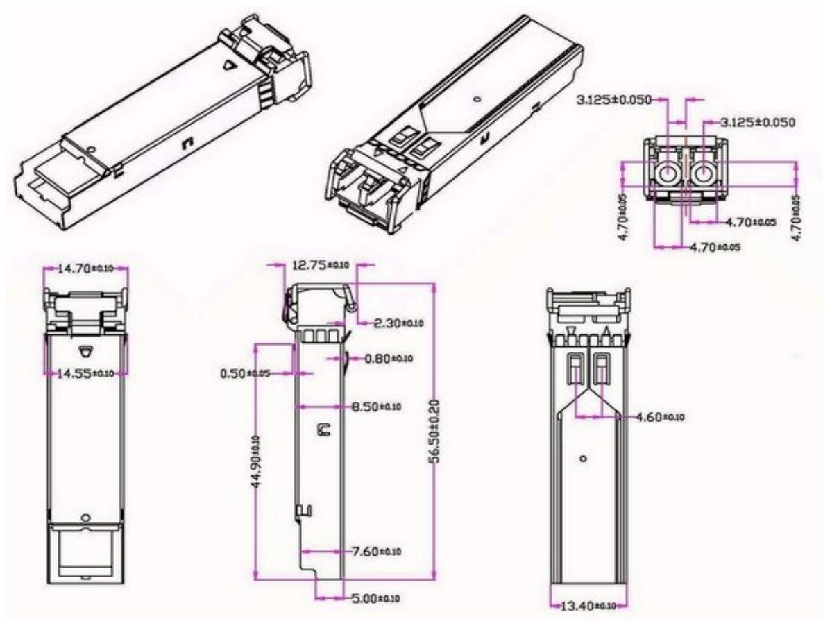
Figure 5, mechanical diagram
